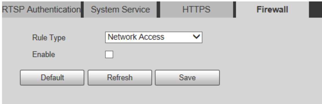
Figure 5-158 Firewall
