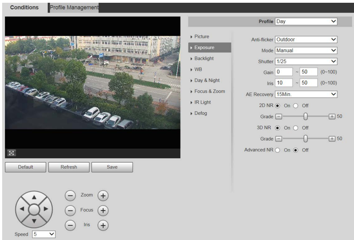
Figure 5-6 Exposure—manual mode
