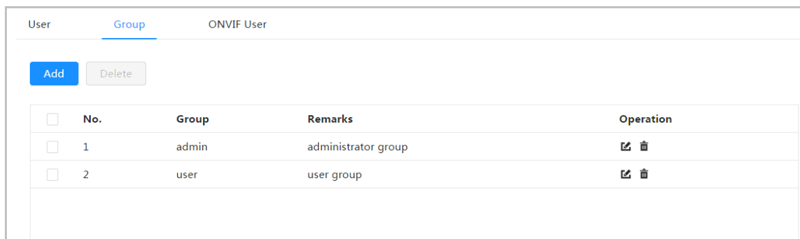
Figure 6-76 Group name
