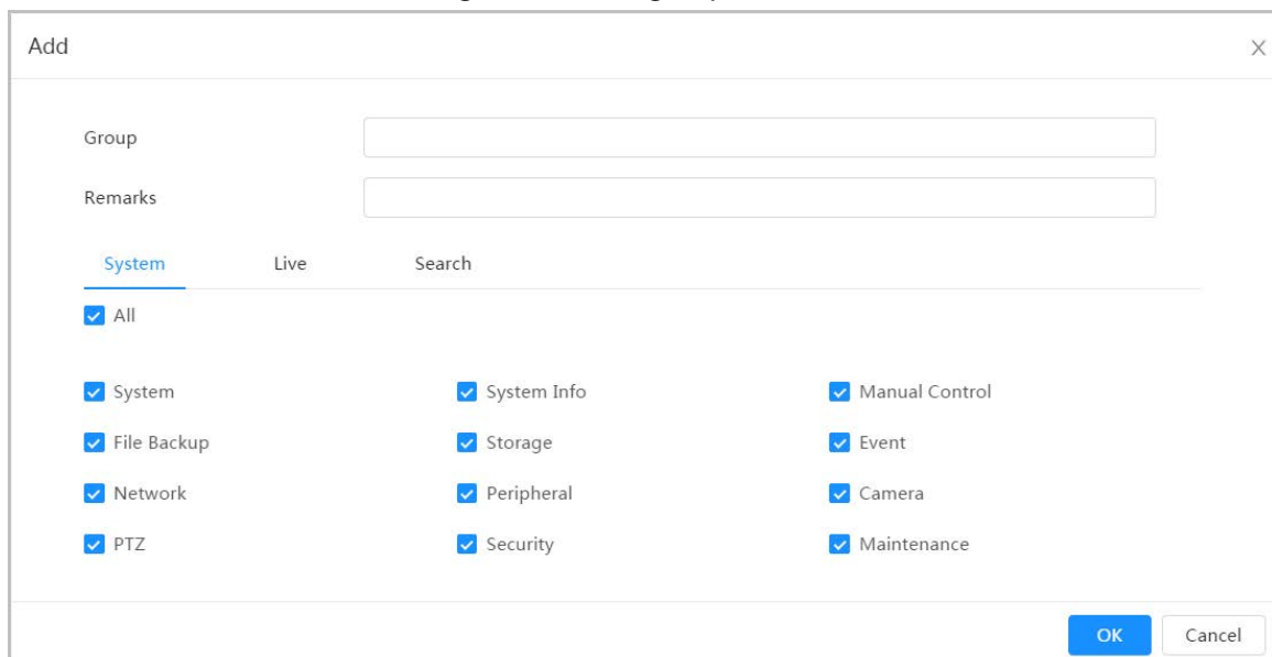
Figure 6-77 Add group
