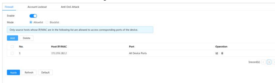
Figure 9-6 Firewall
