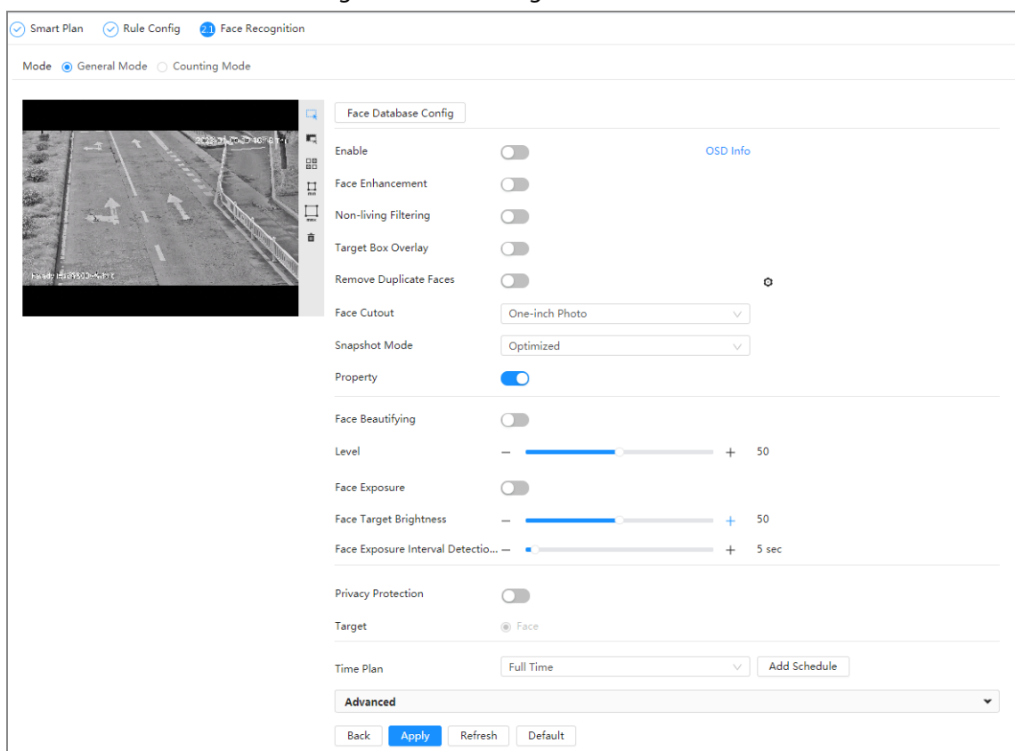
Figure 8-6 Face recognition
