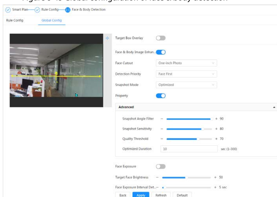
Figure 8-45 Global configuration of face & body detection
