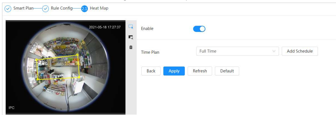
Figure 8-51 Heat Map
