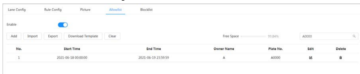
Figure 8-60 Search allowlist
