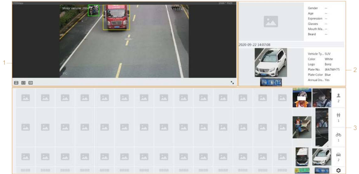
Figure 7-12 Metadata mode
