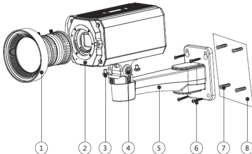
Figure 9-6 Device components
