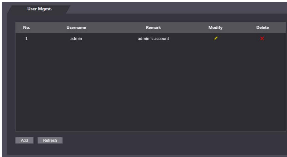
Figure 4-23 User management
