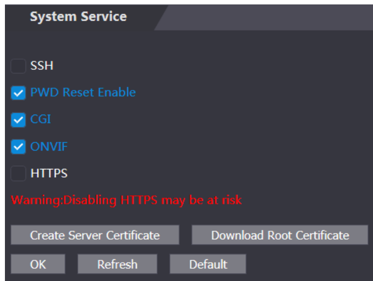
Figure 4-22 System service
