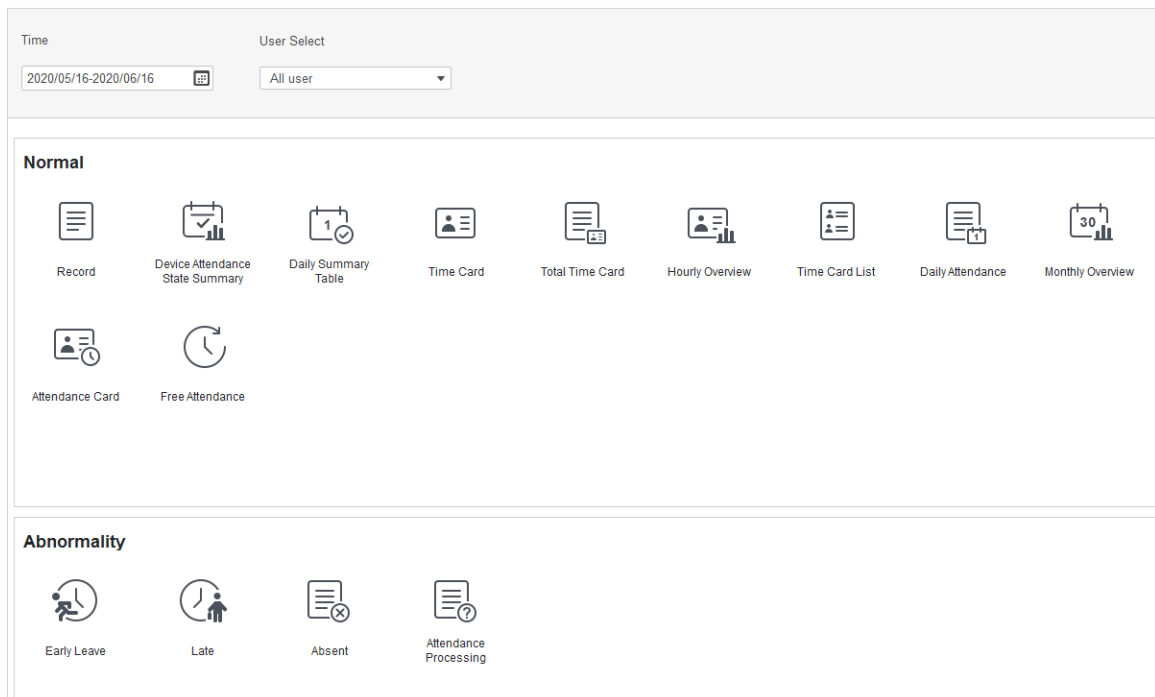
Figure 5-15 Report search
