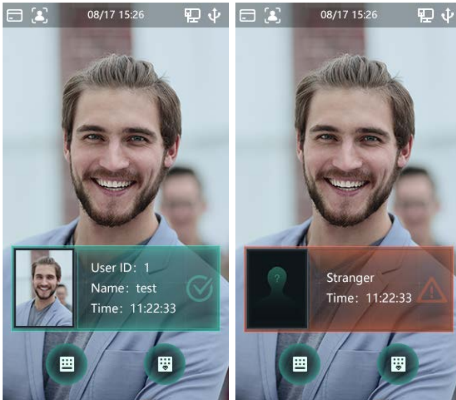
Figure 3-21 Photo&Name mode
