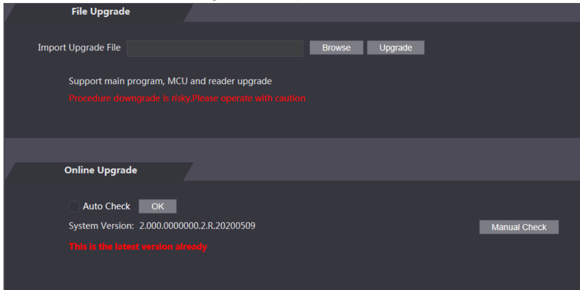
Figure 4-27 Upgrade
