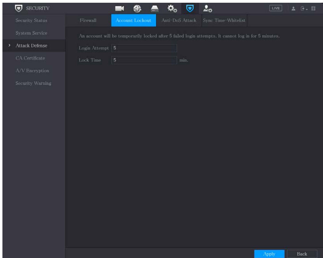
Figure 5-338 Account lockout
