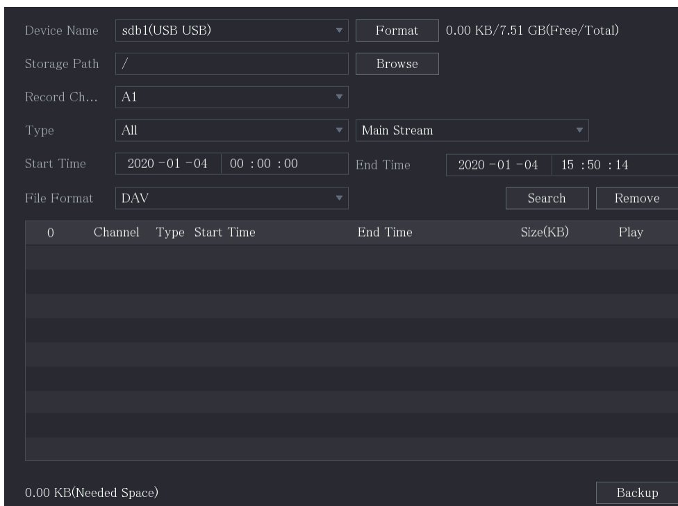
Figure 5-273 Backup
