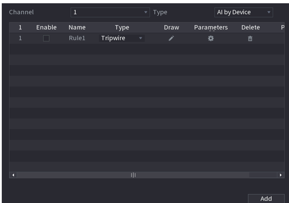
Figure 5-177 Added rule
