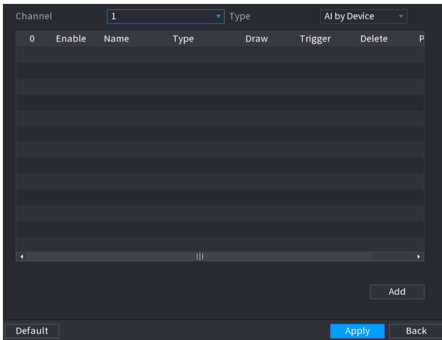
Figure 5-176 IVS
