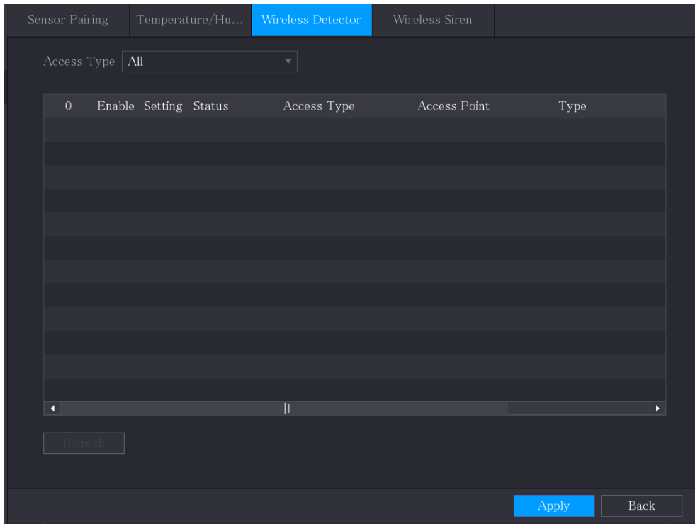
Figure 5-256 Wireless detector
