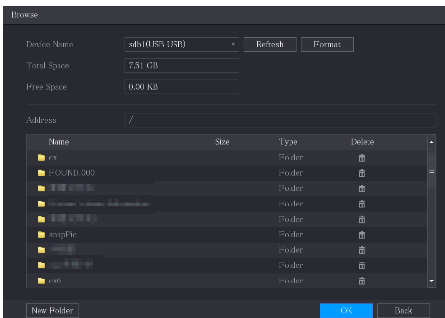
Figure 5-292 Browse
