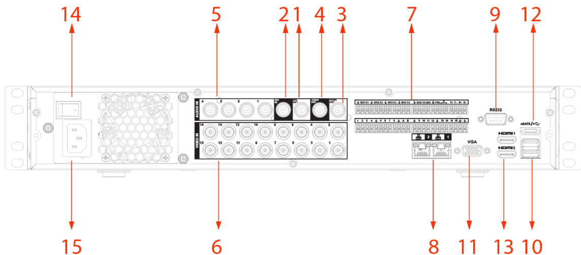
Figure 3-20 Rear panel (3)
