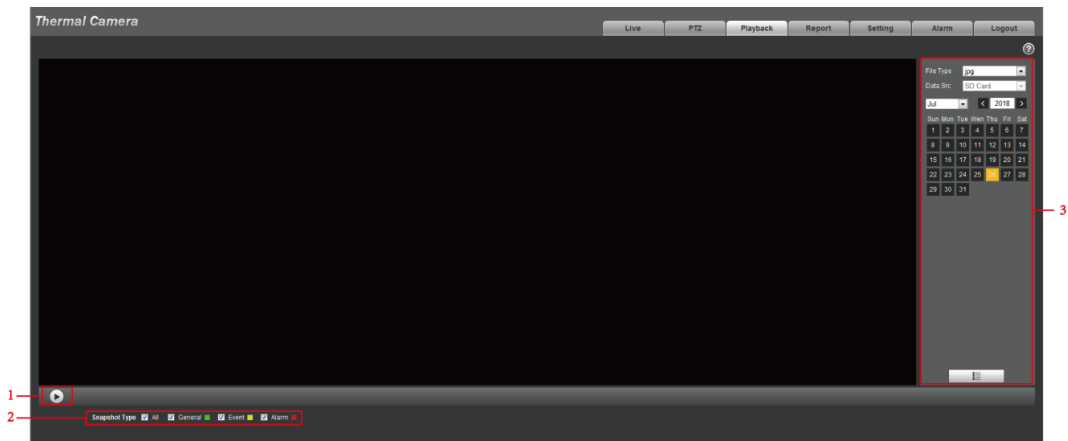
Figure 3-23 Image playback
