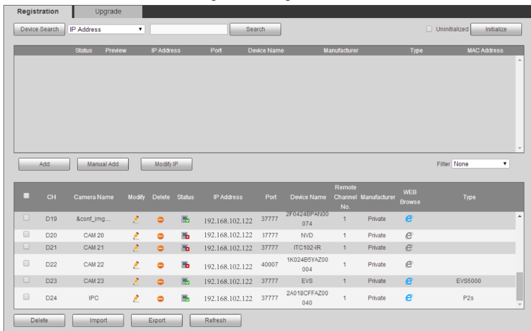
Figure 6-1 Registration
