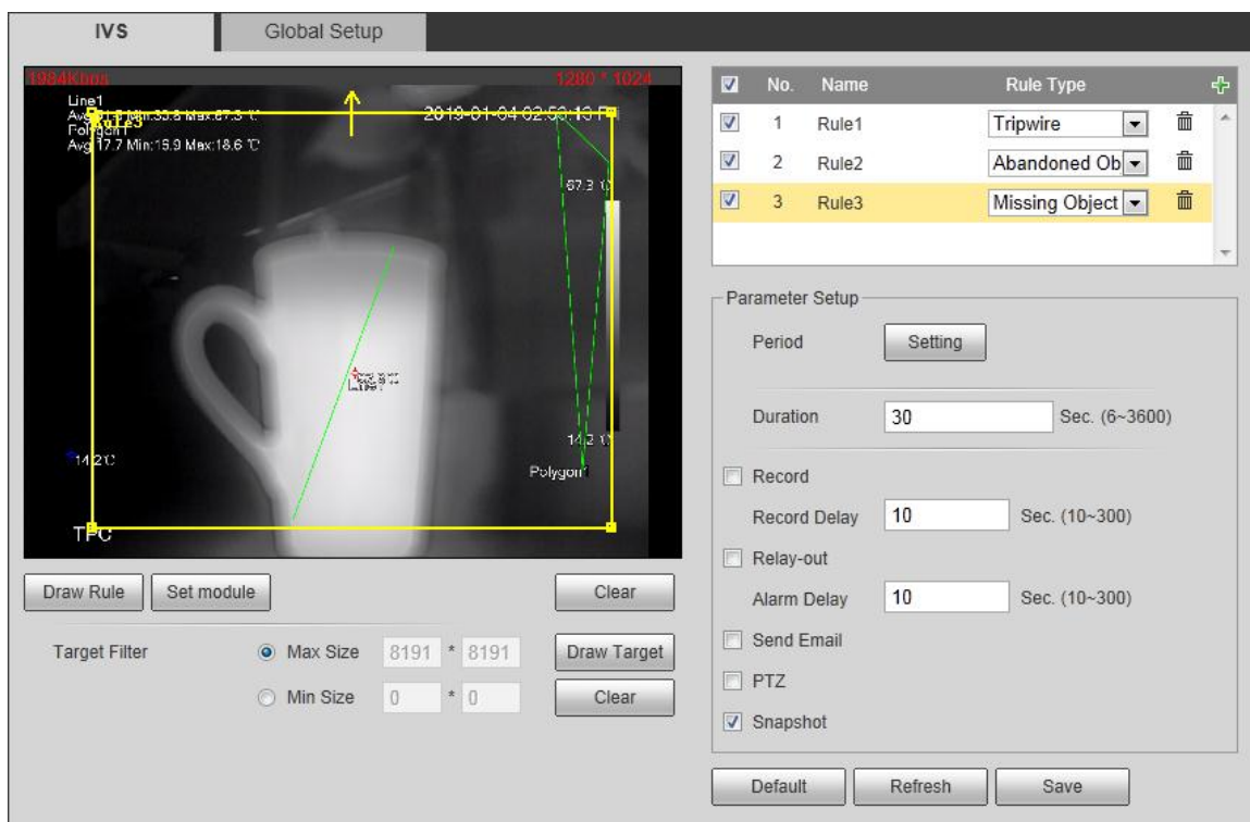
Figure 4-34 Missing object
