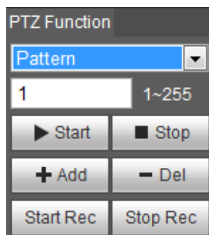
Figure 3-11 Touring pattern
