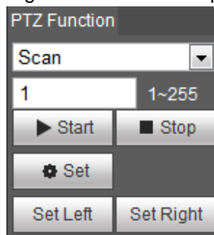
Figure 3-8 Linear sweep
