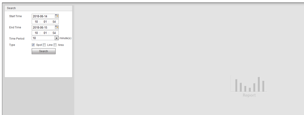
Figure 3-27 Report
