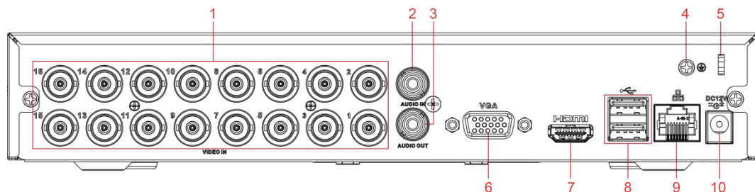
Figure 3-21 Rear panel
