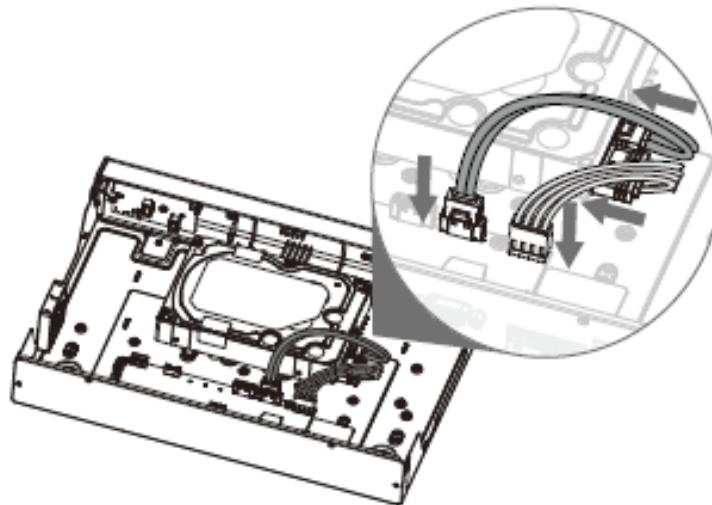
Figure 2-27 Connect cables
