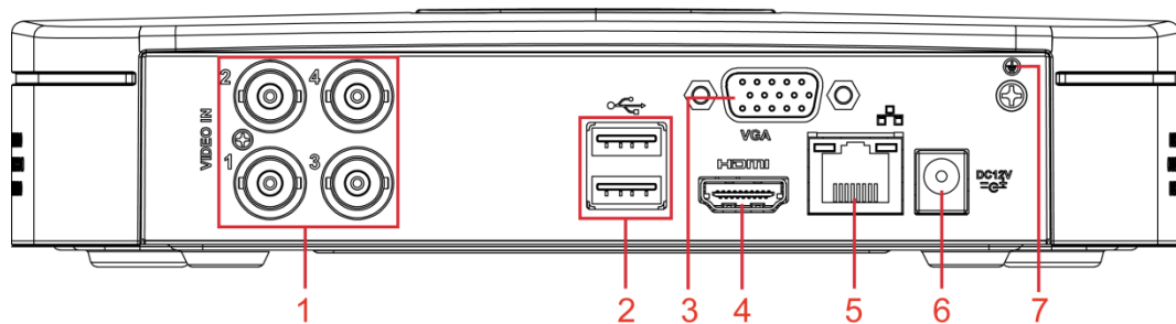
Figure 3-22 Rear panel
