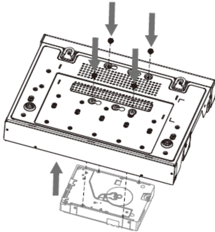
Figure 2-26 Fasten screws
