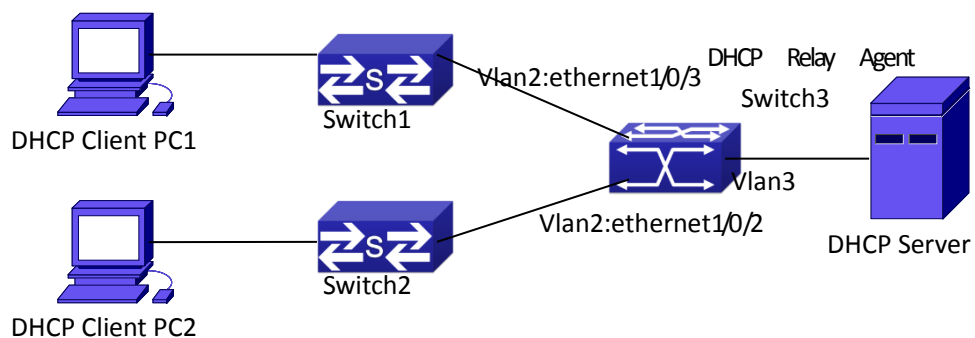
Figure 3-12 A DHCP option 82 typical application example
