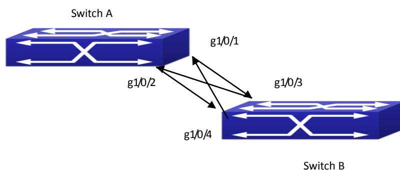
Figure 2-4 Fiber Cross Connection
