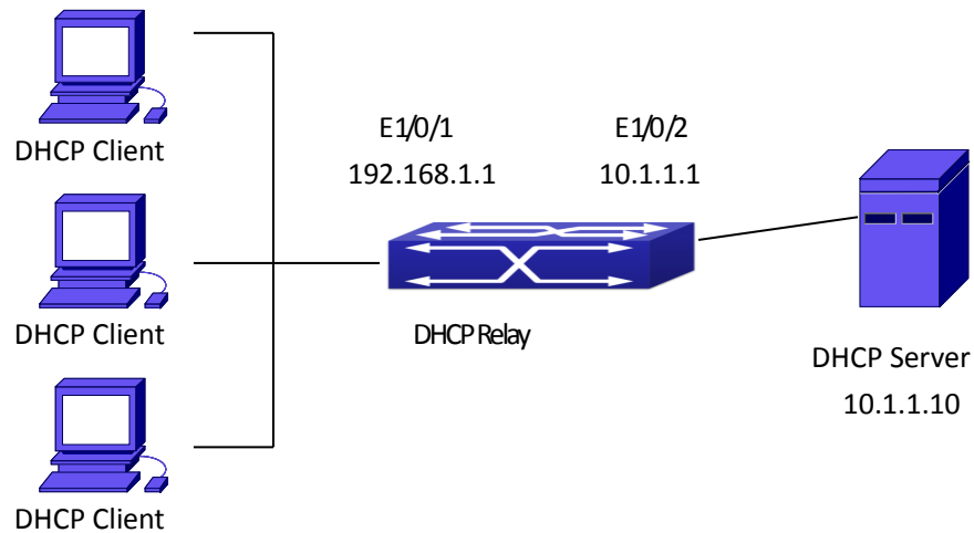
Figure 3-95 DHCP Relay Configuration
