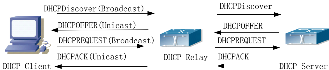
Figure 3-84 DHCP relay
