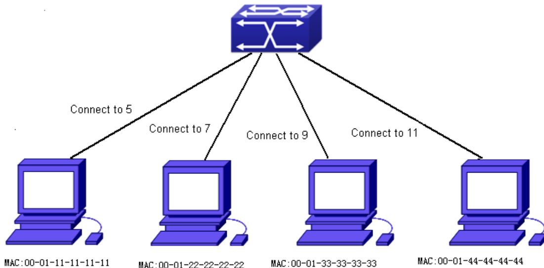
Figure 2-303 MAC Table typical configuration example
