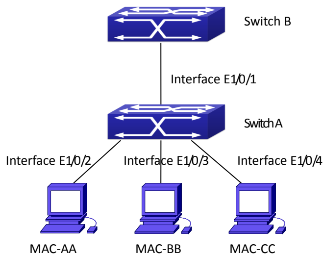
Figure 12-4 DHCPv6 Snooping option schematic
