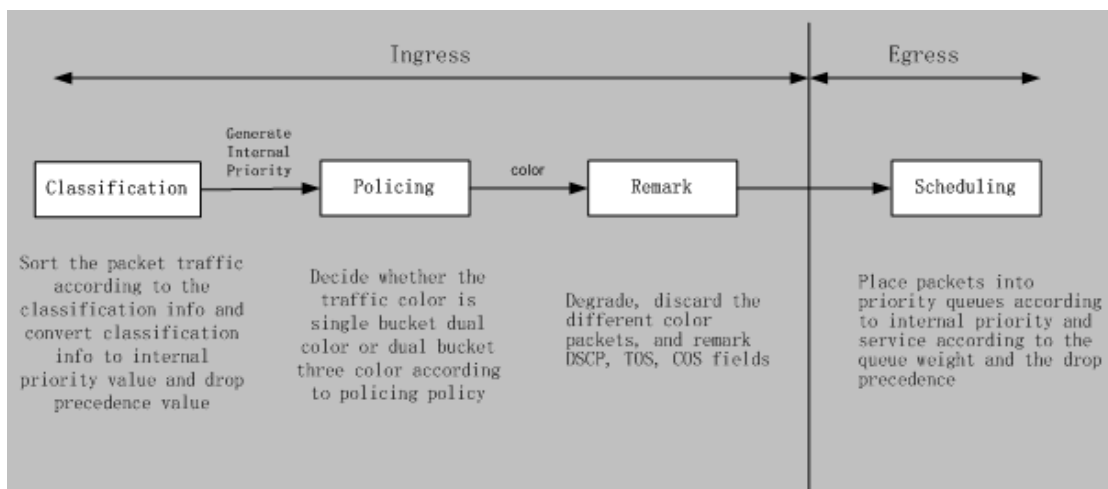
Figure 6-353 Basic QoS Model
