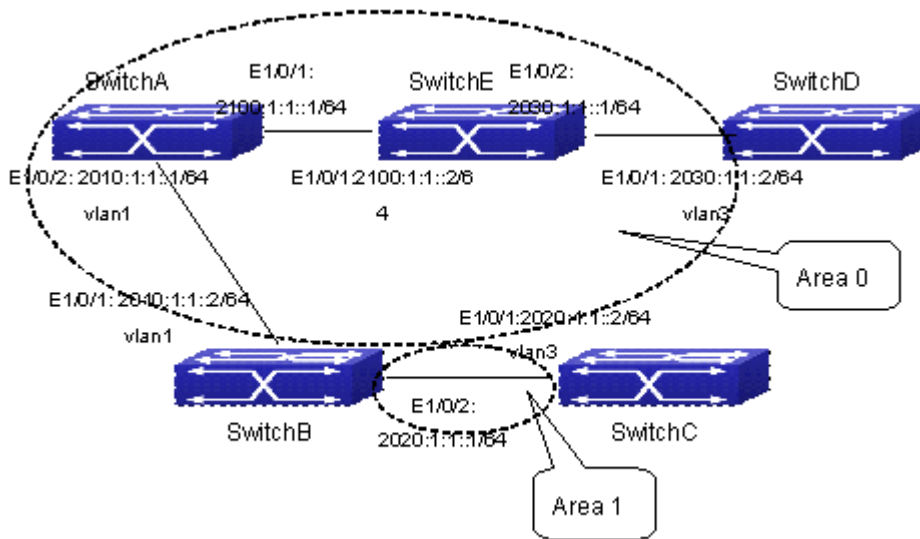
Figure 12-8 Network topology of OSPF autonomous system The configuration for layer3 SwitchA and SwitchE is shown below:
