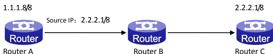
Figure 3-4 URPF application situation
