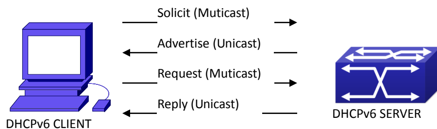
Figure 12-1 DHCPv6 negotiation
