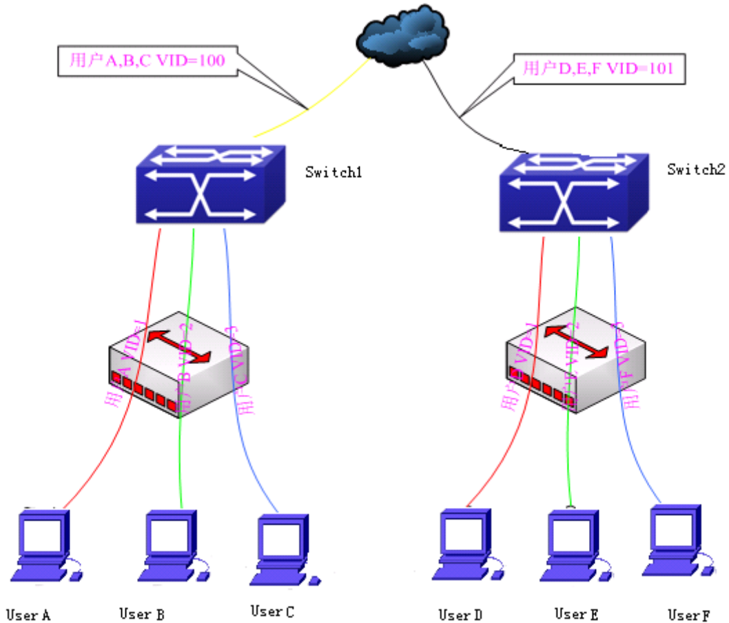
Figure 2-278 VLAN-translation typical application
