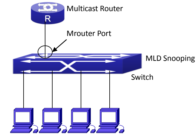
Figure 12-16 Open the Switch MLD Snooping Function figure
