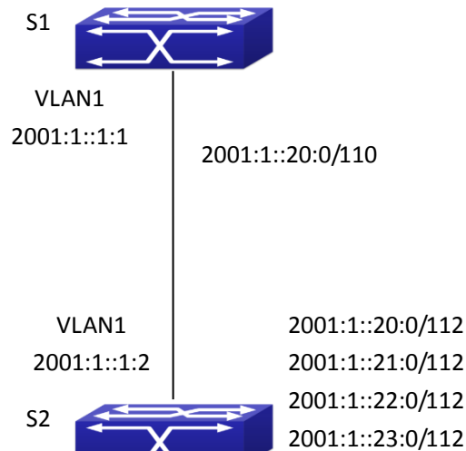
Figure 12-7 Typical application of RIPng aggregation
