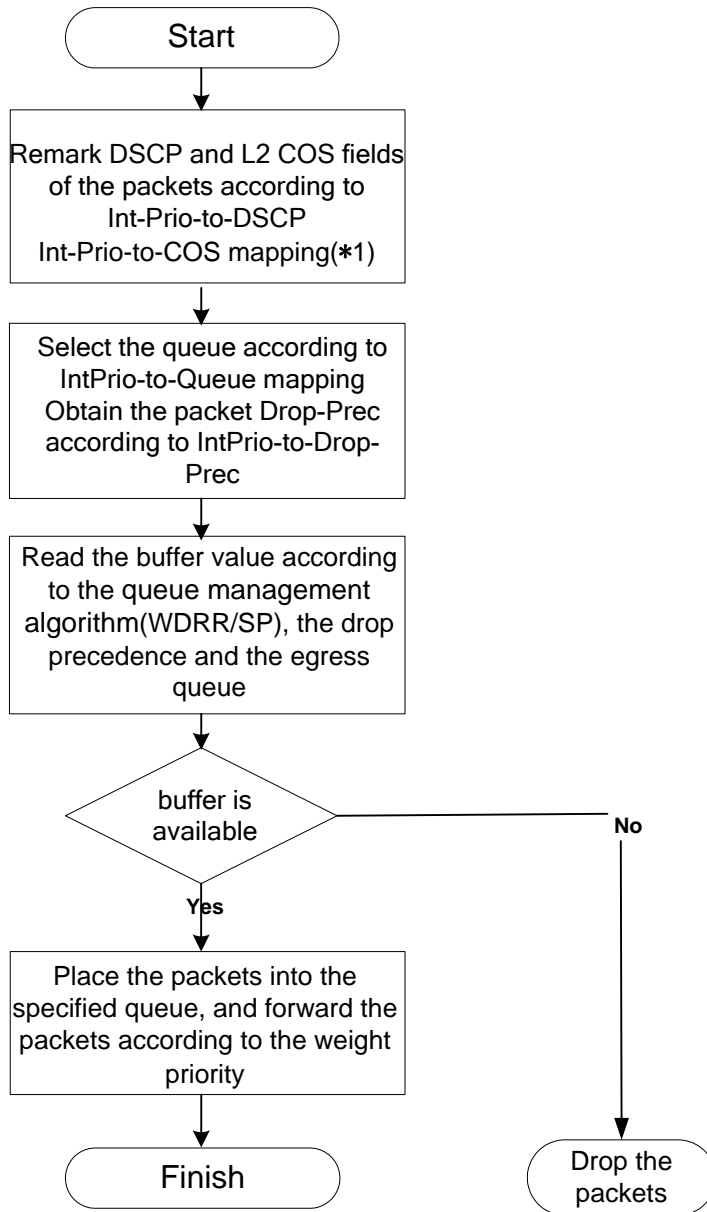
Figure 6-386 Queuing and Scheduling process
