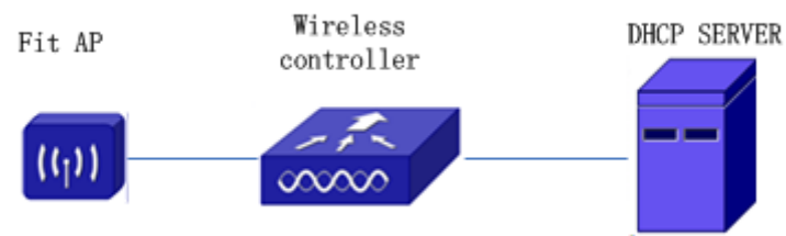
Figure 3-14 Typical DHCP option 60 and option 43 topology
