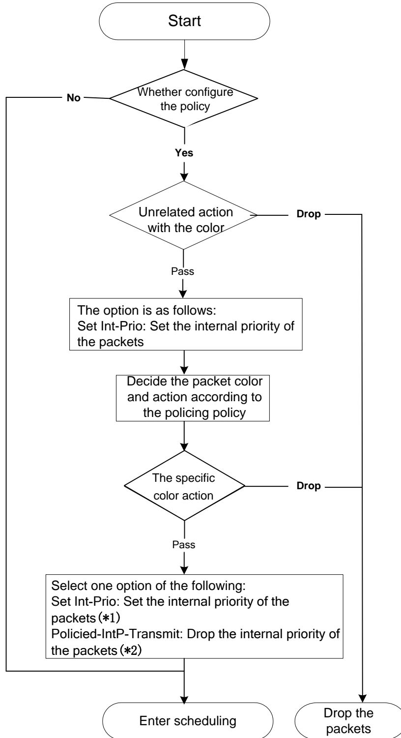
Figure 6-375 Policing and Remarking process
