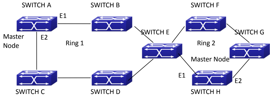
Figure 7-7 MRPP Sketch Map
