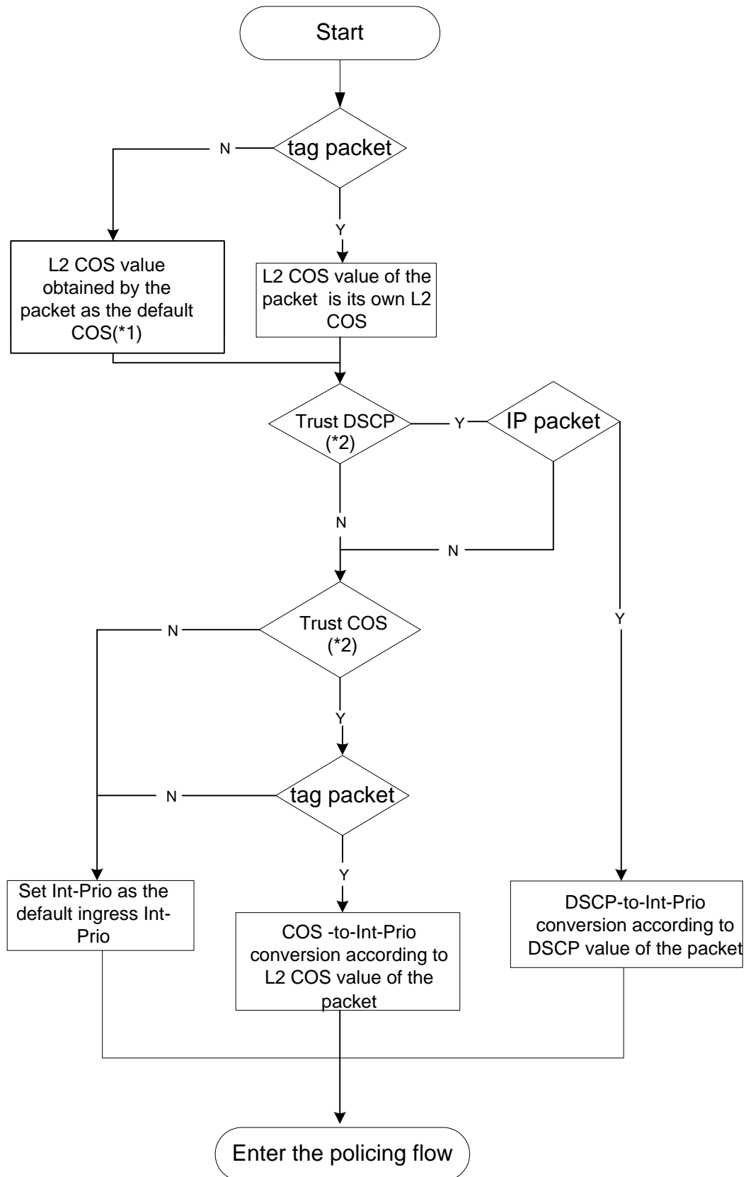
Figure 6-364 Classification process
