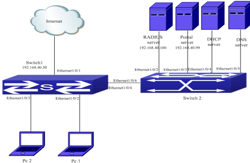
Figure 6-271 Automatic Page Pushing after Successful Authentication Configuration Configuration steps:
