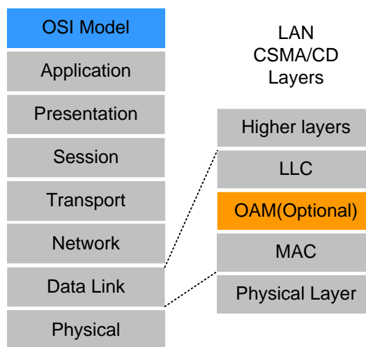
Figure 2-154 OAM location in OSI model
