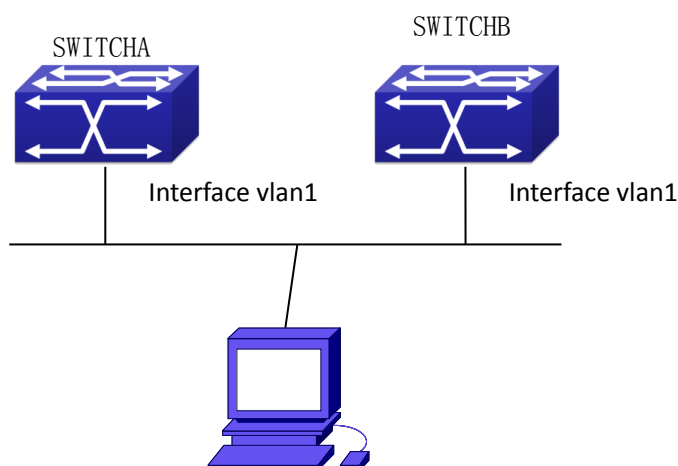
Figure 7-6 VRRP Network Topology
