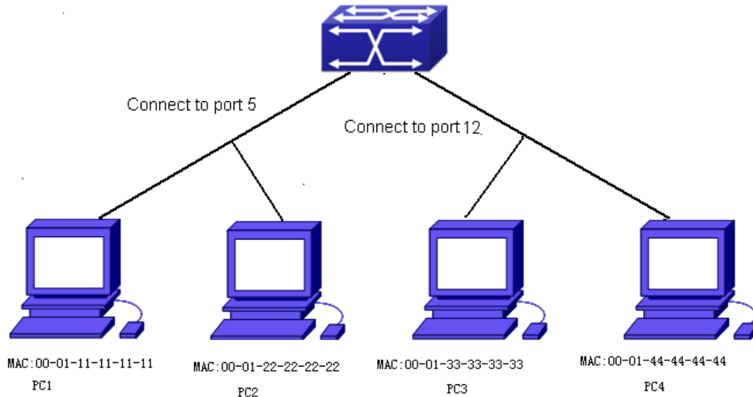
Figure 2-292 MAC Table dynamic learning
