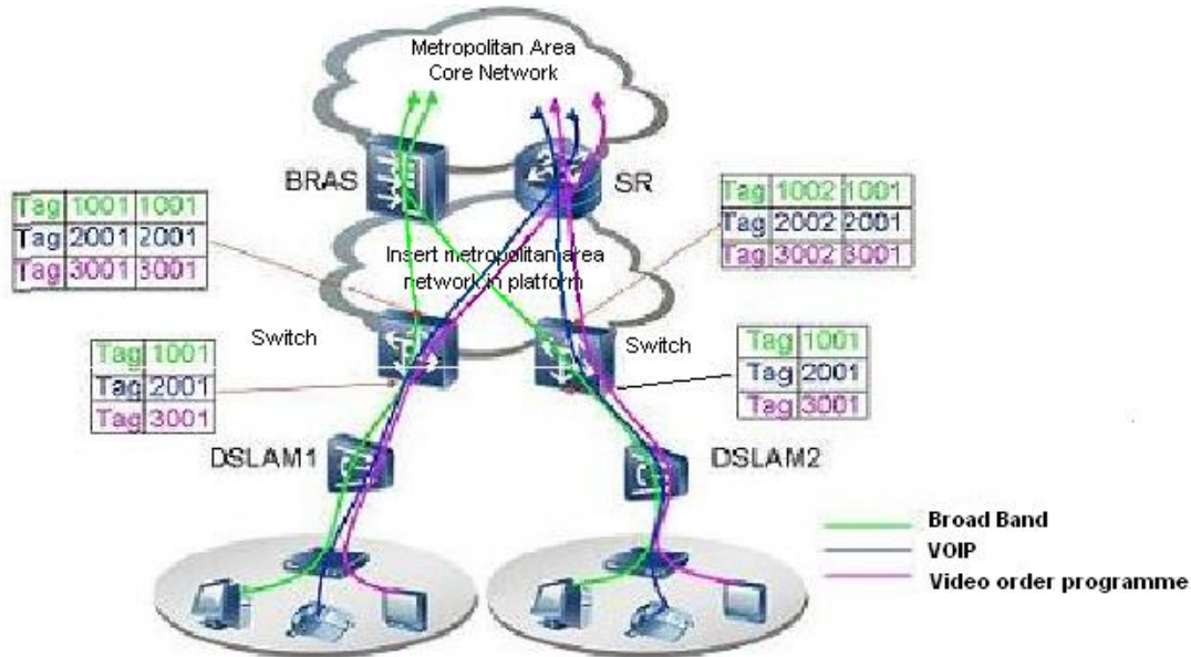
Figure 6-390 Flexible QinQ application topology
