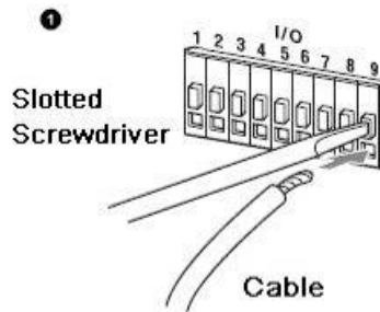
Figure 9-4 Install cable
