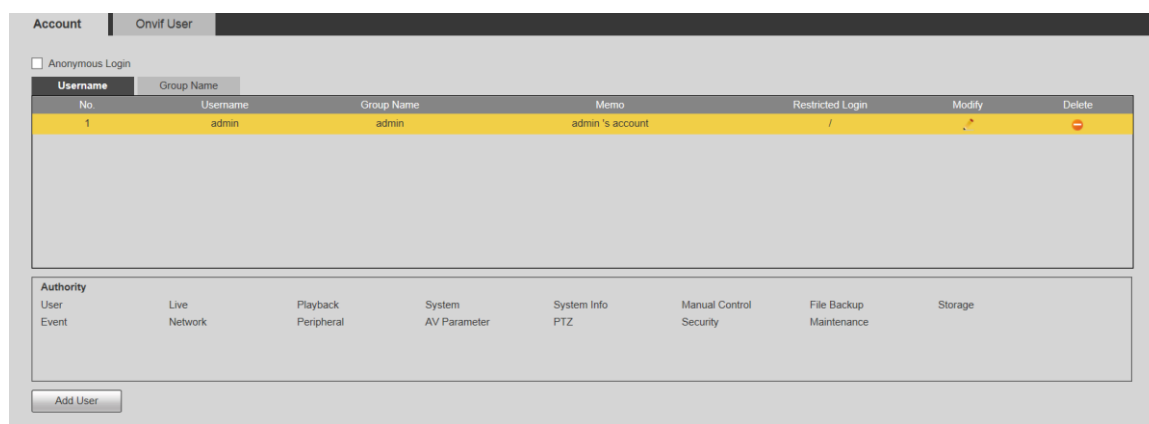
Figure 5-137 Account interface
