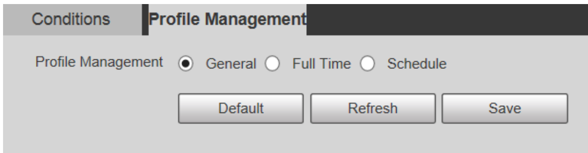
Figure 5-19 Profile management—general
