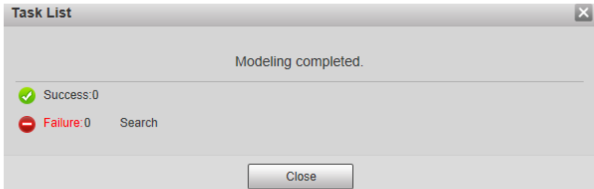
Figure 5-105 Modeling completed
