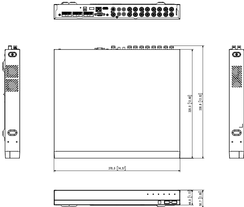
Appearance drawing HRX-1634 Unit : mm[inches]
