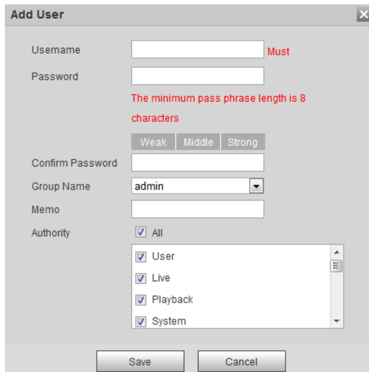
Figure 4-90 Add user
