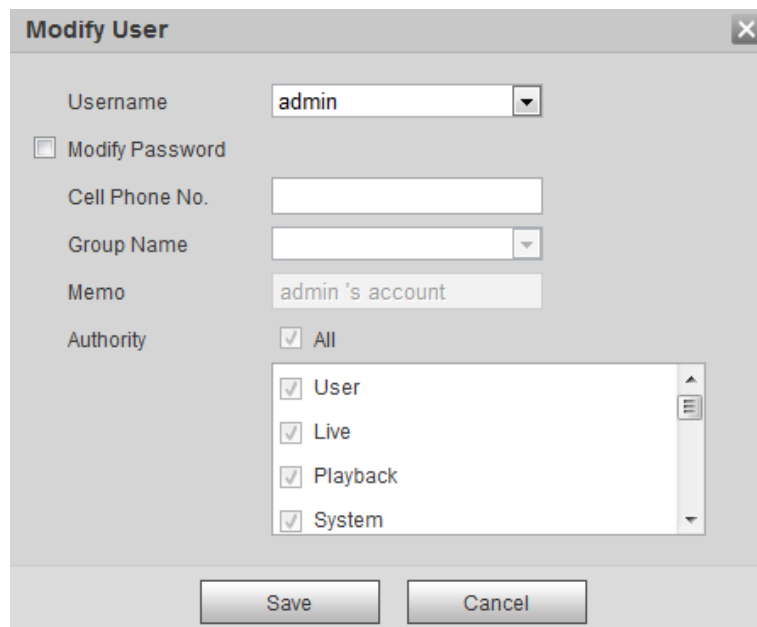
Figure 4-92 Modify user (1)
