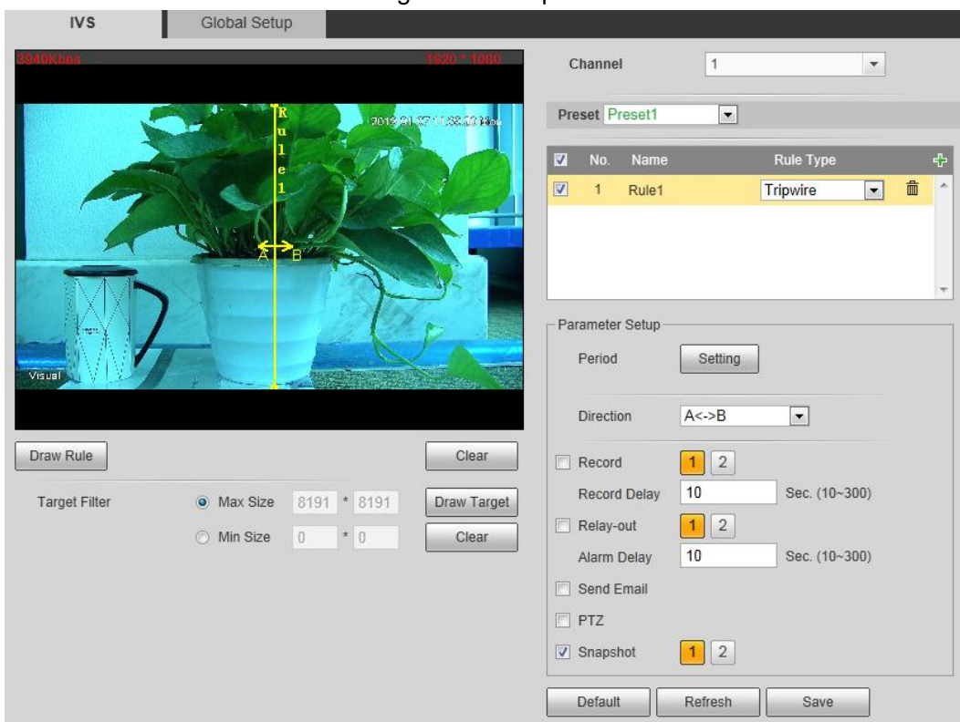
Figure 4-43 Tripwire
