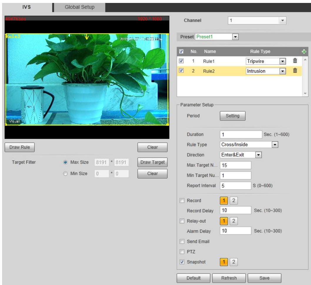
Figure 4-44 Intrusion
