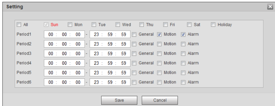
Figure 4-74 Setting
