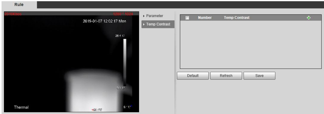
Figure 4-66 Temperature contrast
