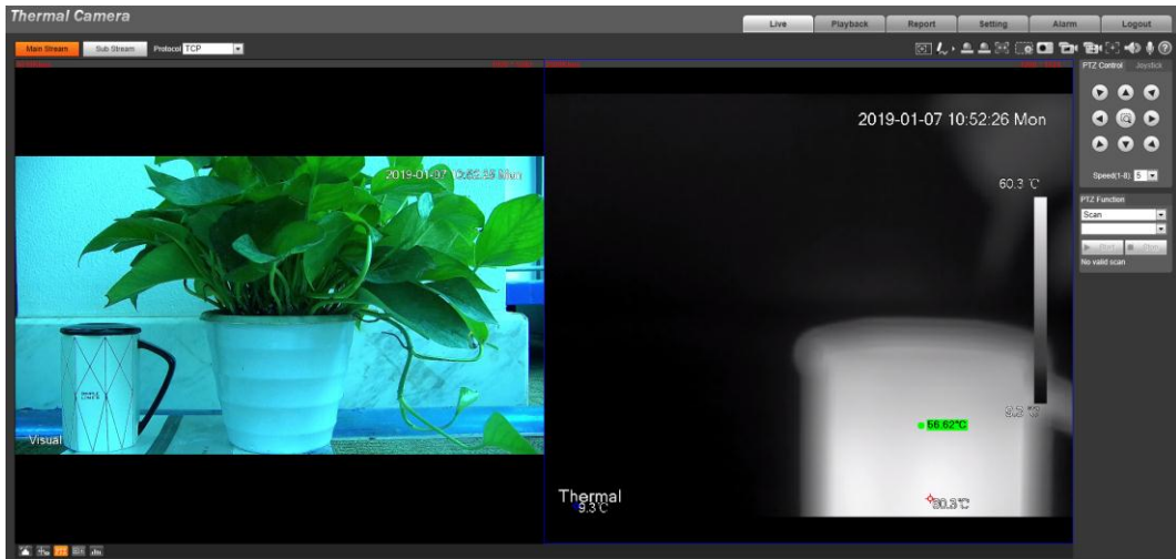
Figure 2-5 Live Interface
