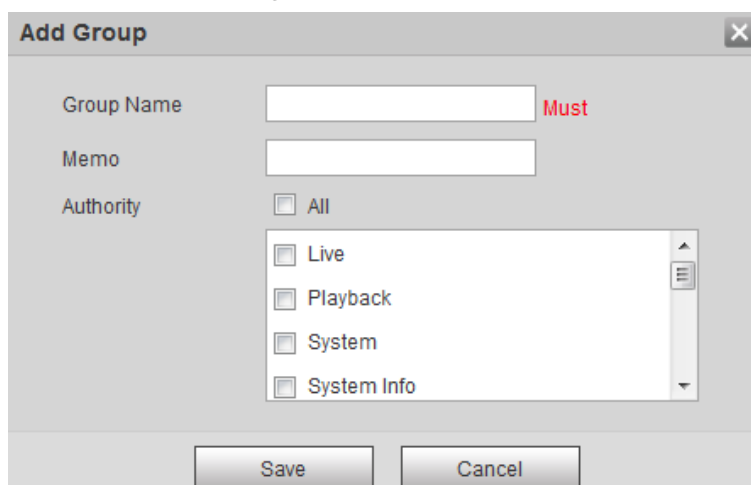
Figure 4-87 Add Group
