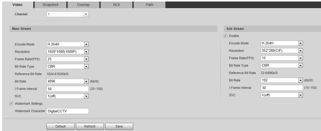
Figure 4-13 Video
