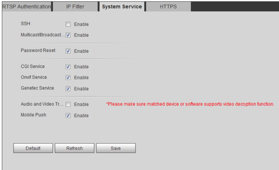
Figure 4-98 System service
