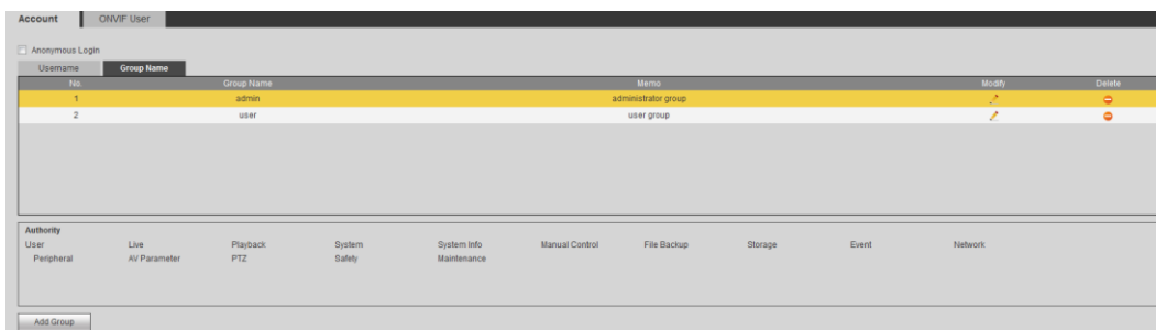
Figure 4-86 User group
