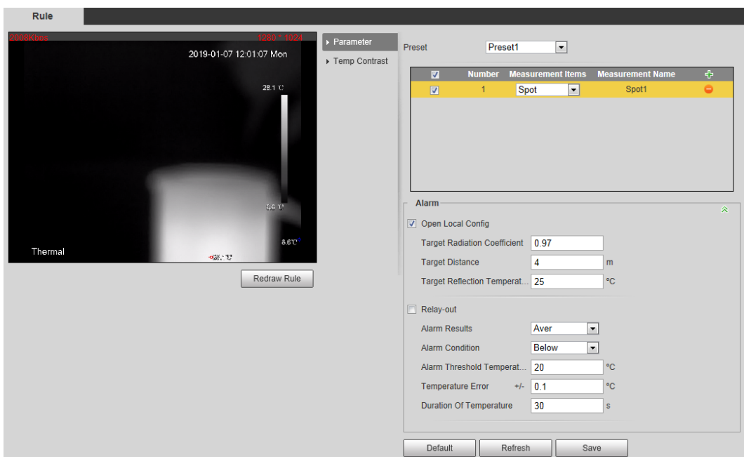
Figure 4-65 Rule adding
