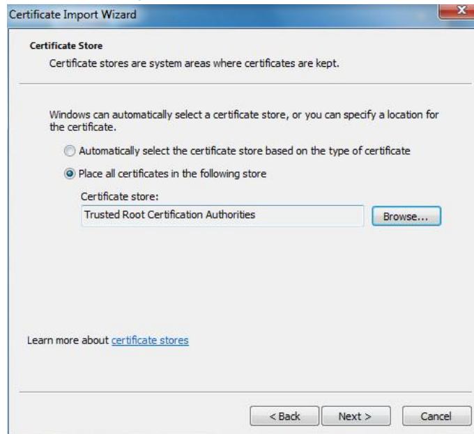
Figure 4-110 Certificate store
