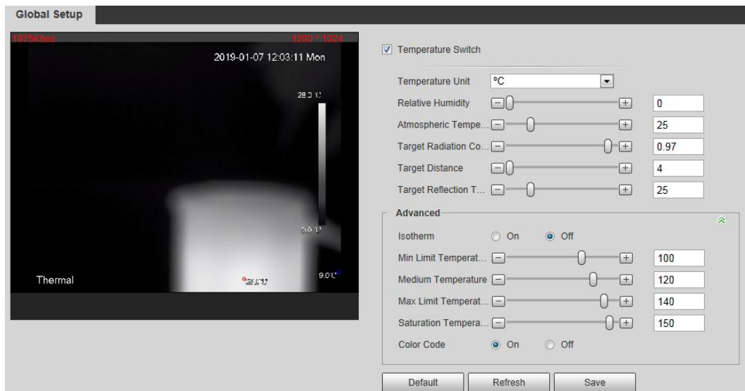
Figure 4-68 Global setup
