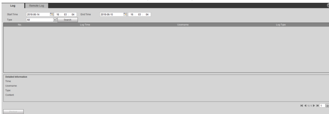
Figure 5-7 Log
