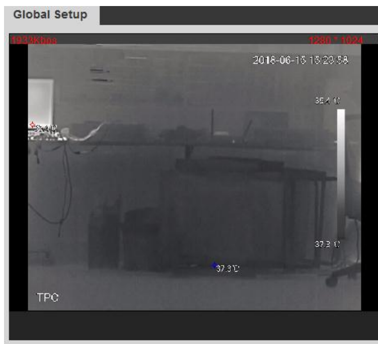
Figure 4-71 Color code
