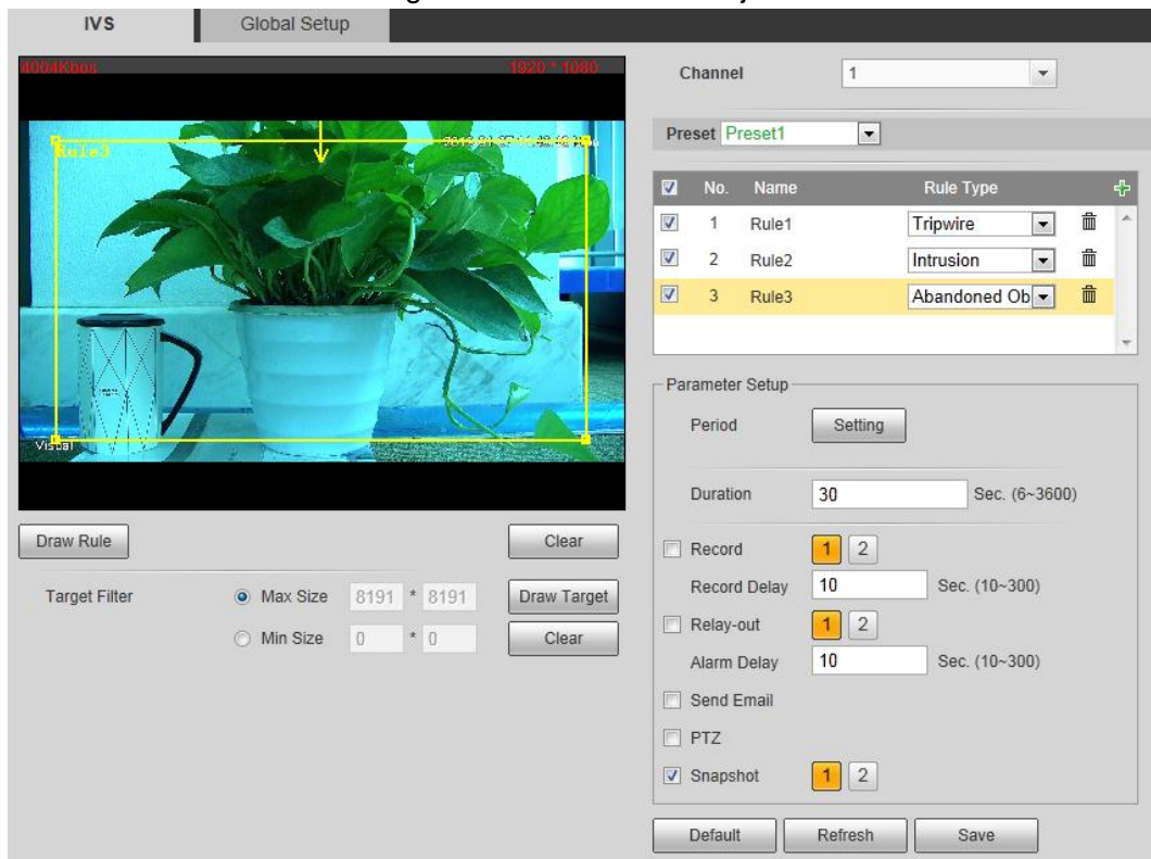
Figure 4-45 Abandoned object
