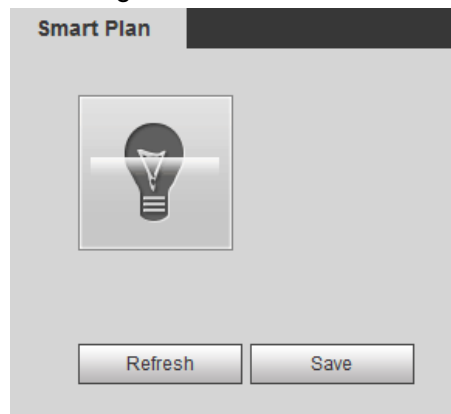
Figure 4-42 Smart Plan
