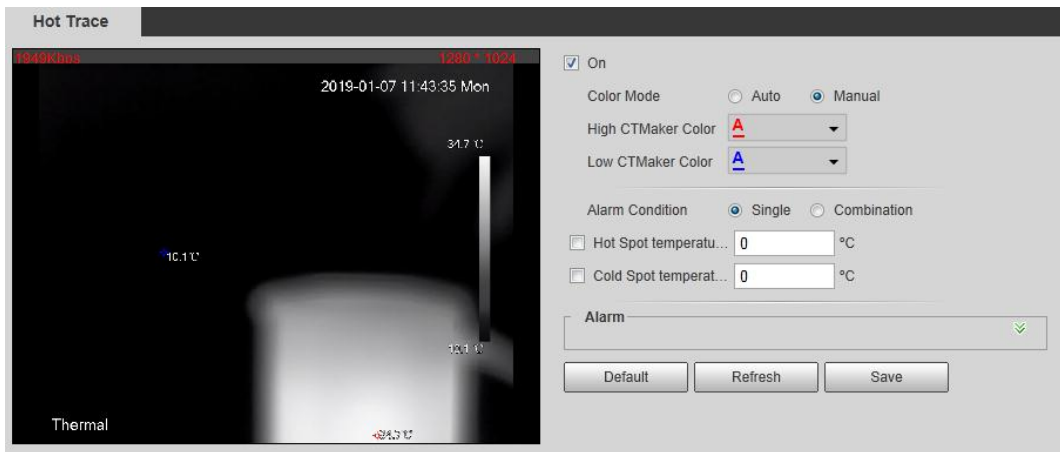
Figure 4-49 Hot trace
