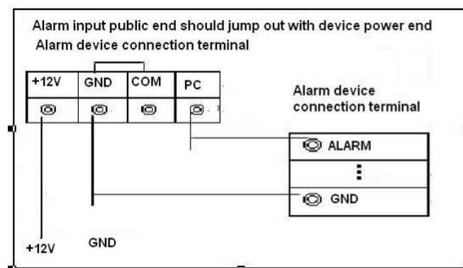
Figure 4-3 Alarm input
