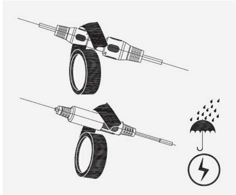
Figure 10-4 Waterproof measures
