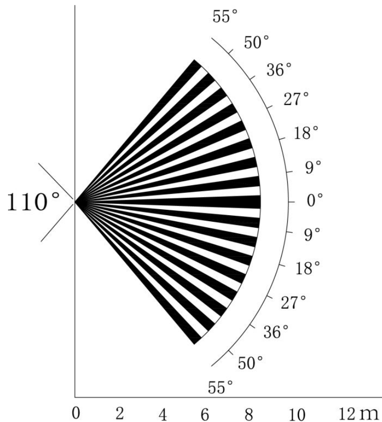
Figure 7-1 Horizontal detection range
