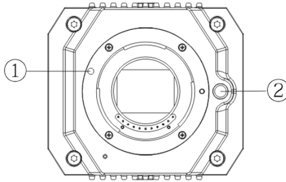
Figure 8-2 Front panel
