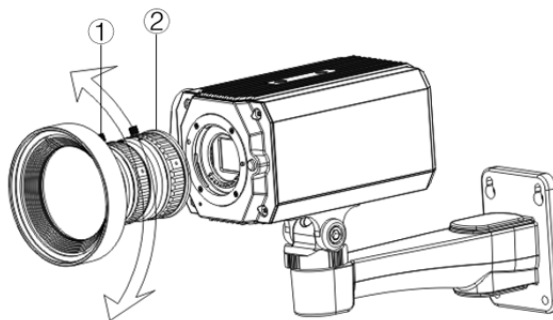
Figure 8-3 Lens installation (2)
