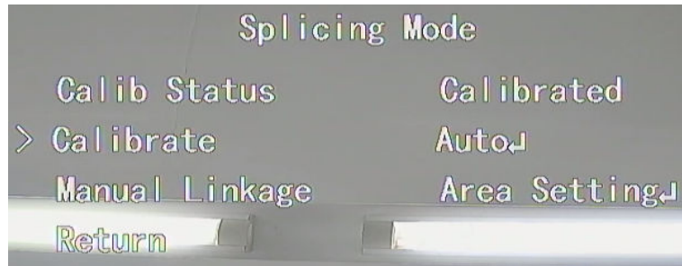
Figure 6-11 Manual linkage
