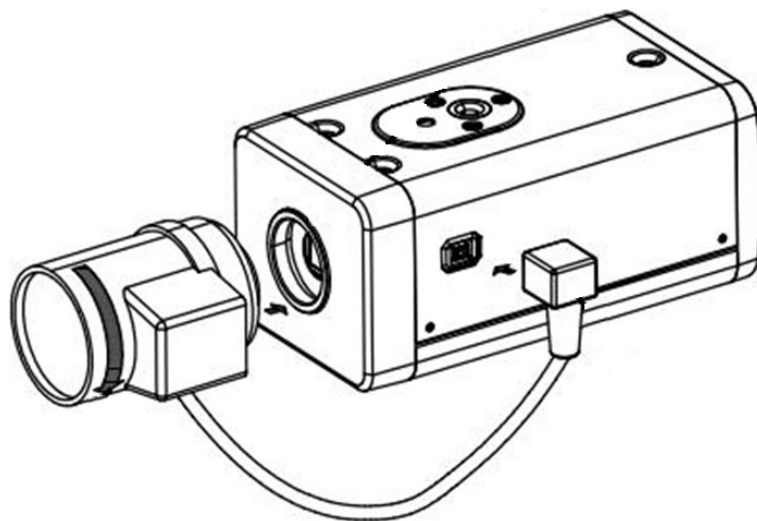
Figure 8-1 Lens installation (1)
