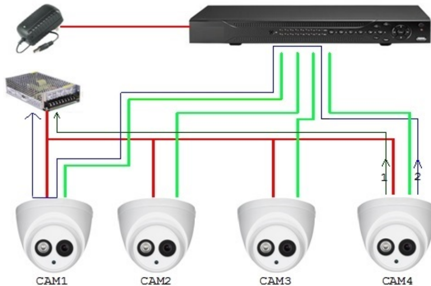
Figure 10-3 Principle of centralized power supply
