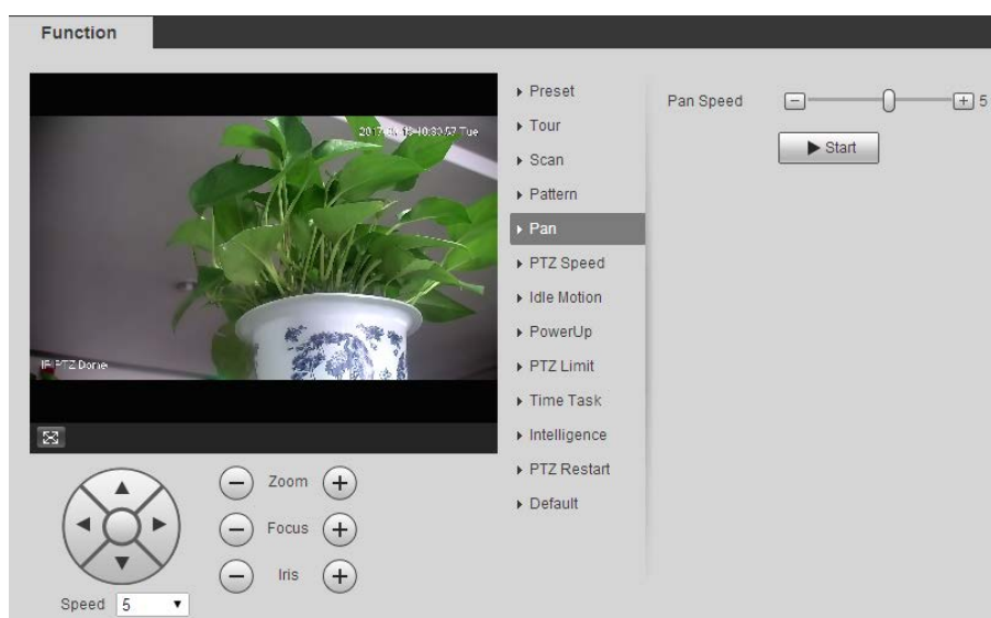
Figure 5-70 Pan settings
