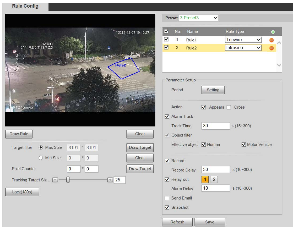
Figure 5-91 Intrusion settings
