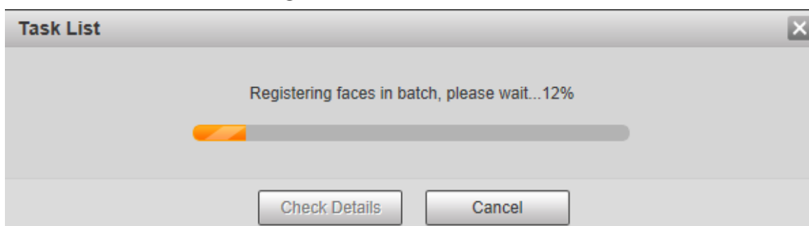
Figure 5-104 Registering
