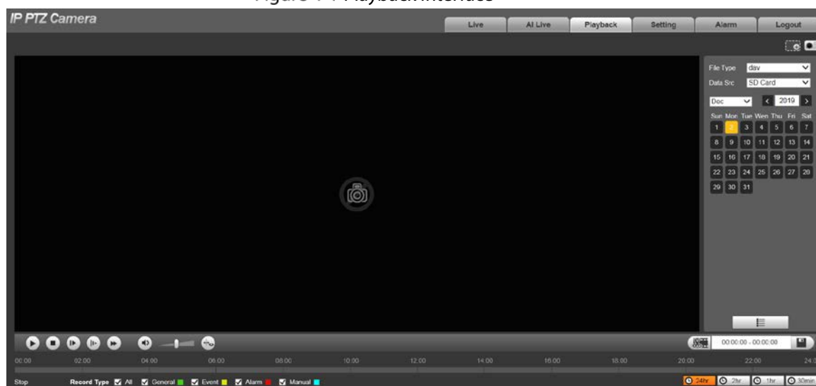
Figure 4-1 Playback interface
