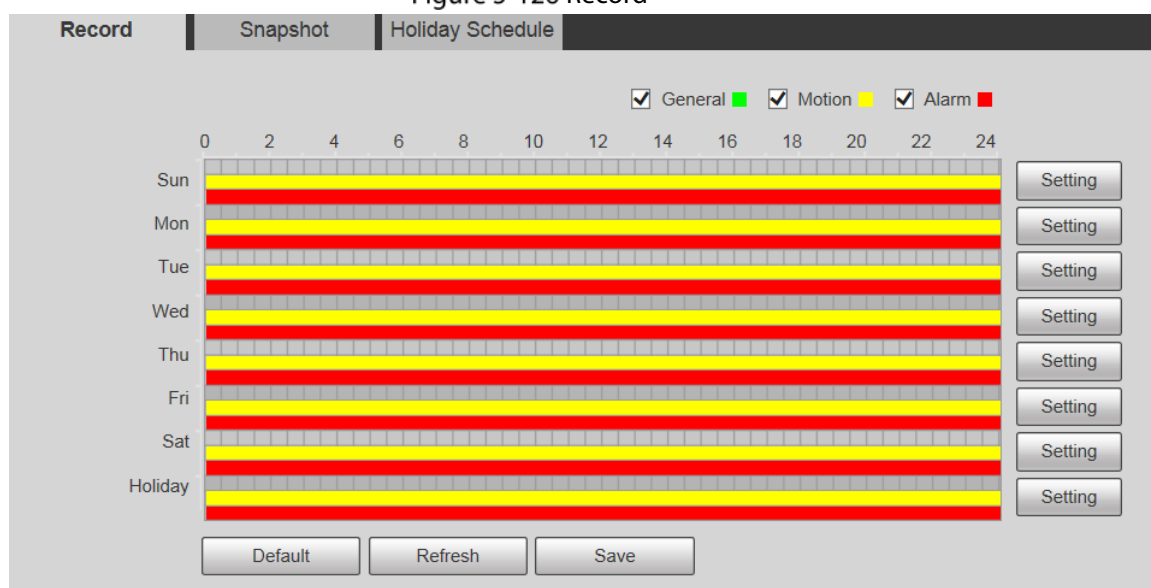
Figure 5-126 Record
