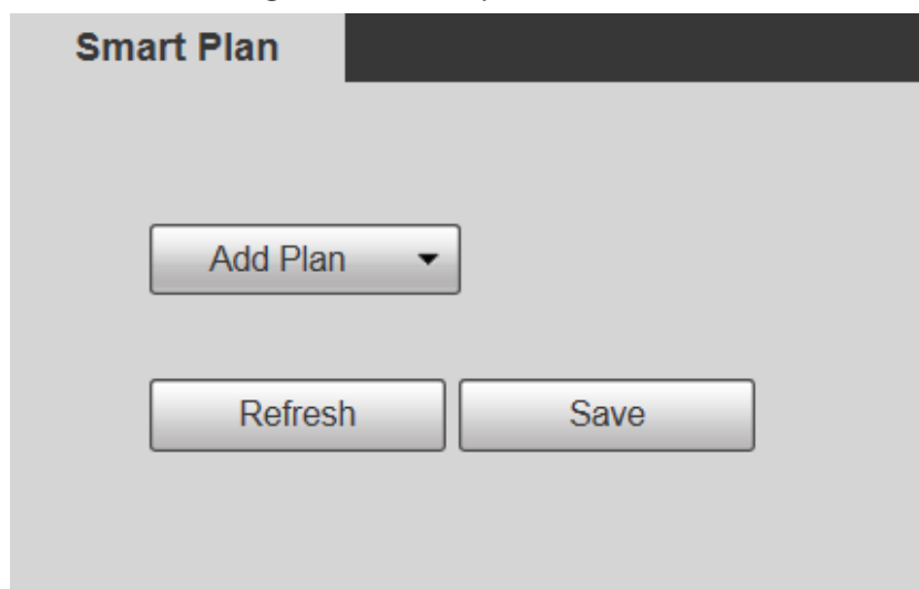
Figure 5-86 Smart plan (1)
