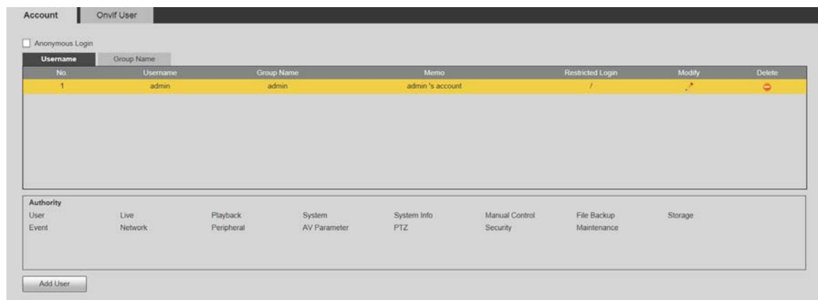
Figure 5-139 Account interface
