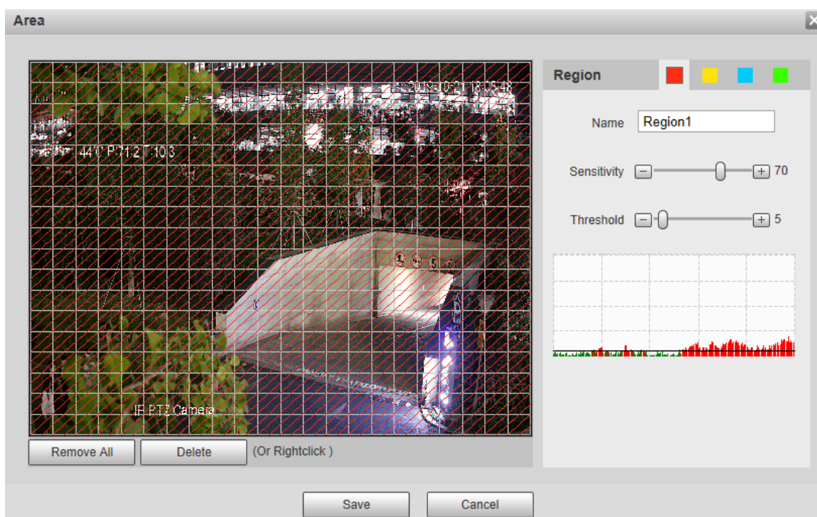
Figure 5-81 Area setting
