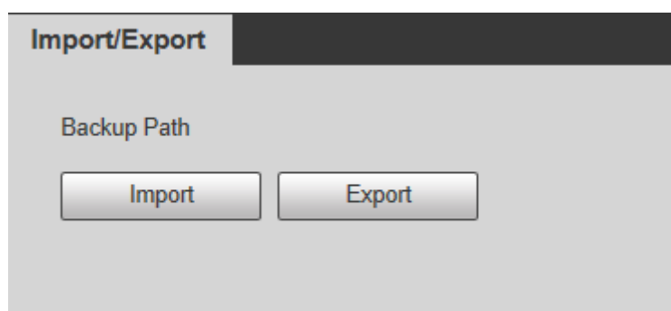
Figure 5-163 Import/Export
