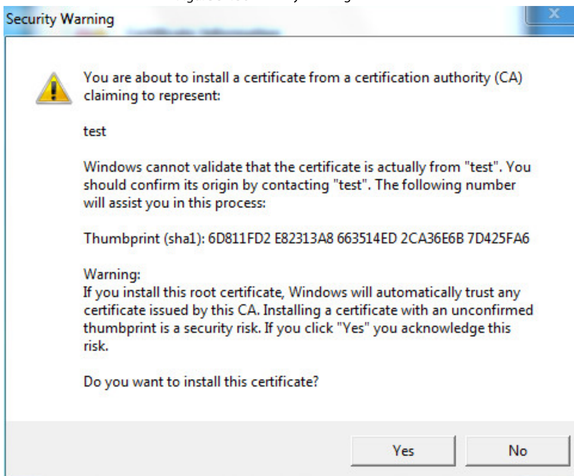
Figure 5-156 Security warning
