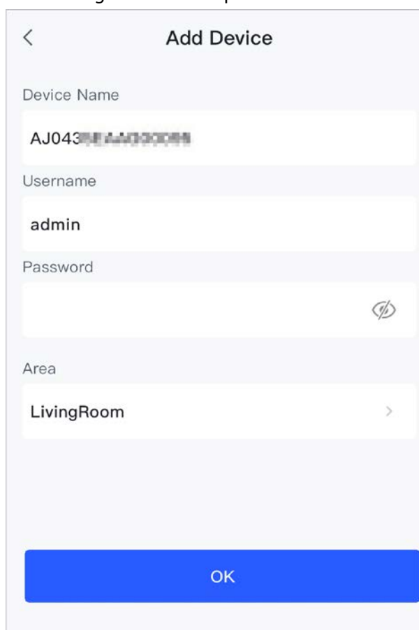
Figure 4-10 Enter password
