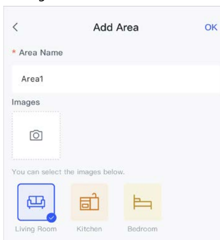
Figure 4-18 Add area
