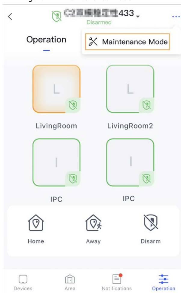
Figure 4-22 Maintenance mode
