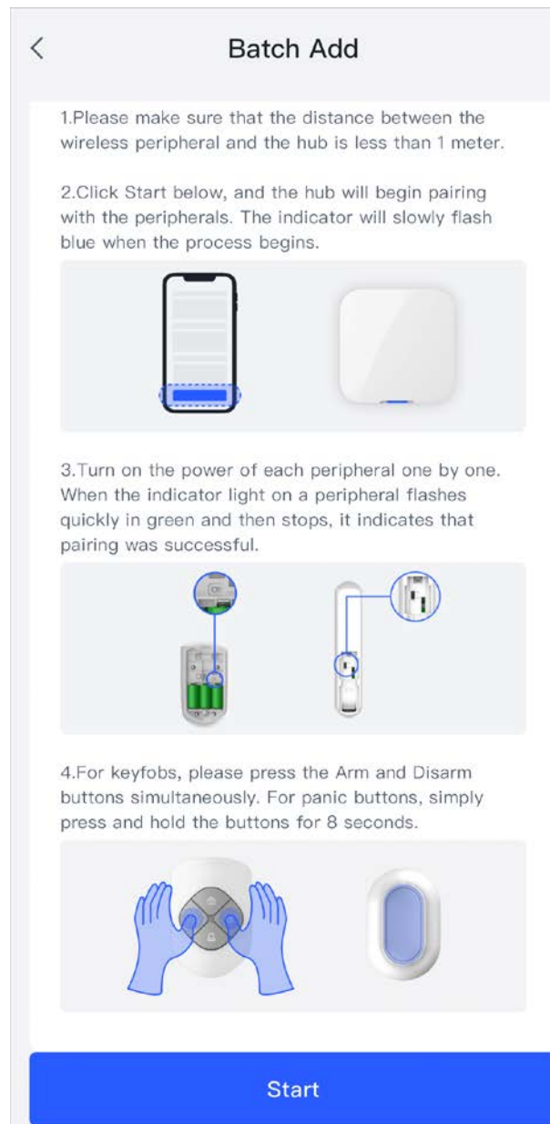
Figure 4-6 Batch add
