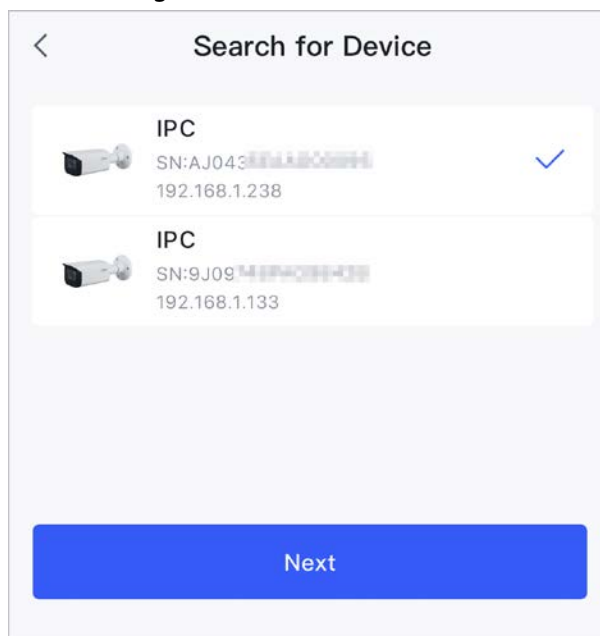
Figure 4-9 Online search
