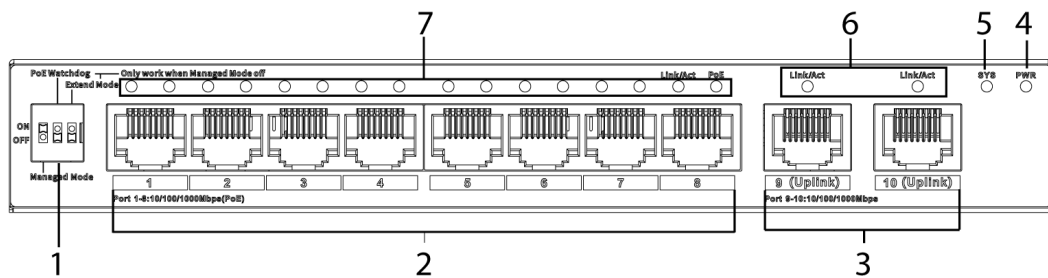
Figure 2-1 Front panel
