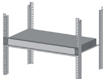
Figure 3-2 Fix the Device onto the rack
