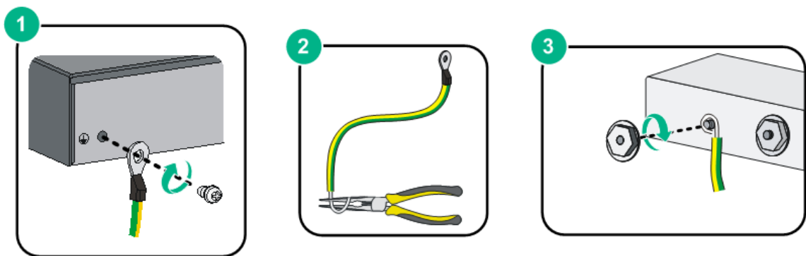
Figure 4-1 Connect GND
