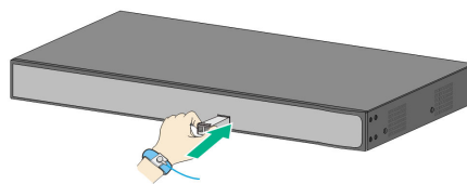
Figure 4-4 Install SFP module
