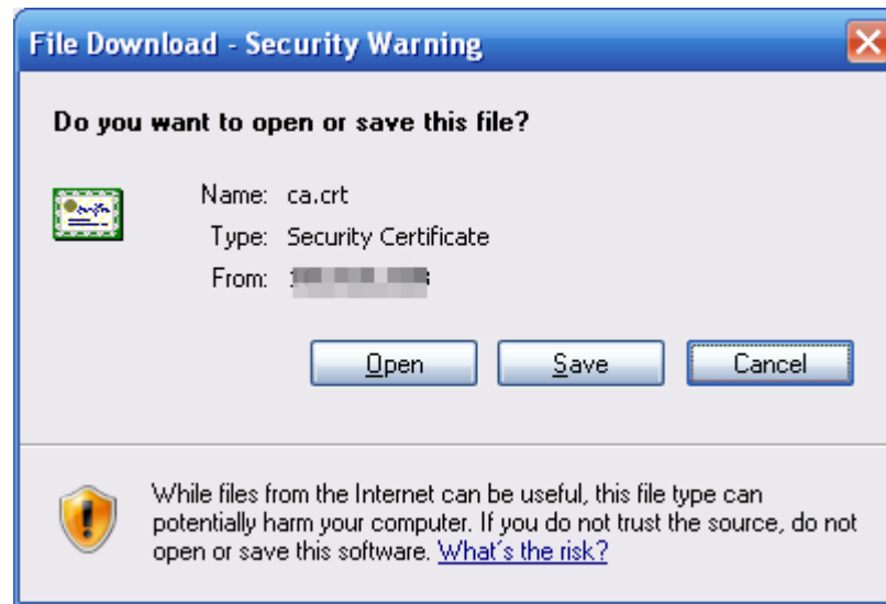
Figure 4-117 File download
