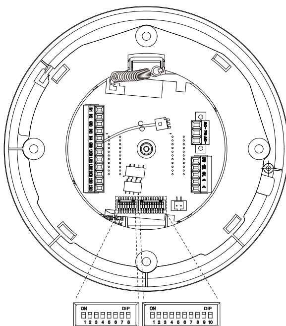
Camera ID DIP Switch (SW2) Communication Protocol DIP Switch (SW1)
