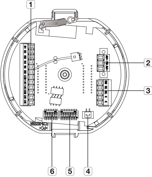
Inner View of Installation Base
