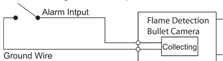
Figure 1-2 Alarm input
