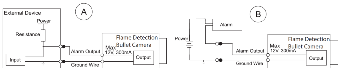
Figure 1-3 Alarm output
