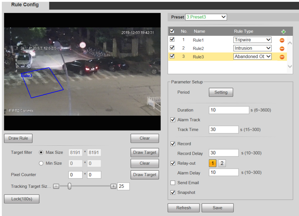
Figure 5-95 Abandoned object settings
