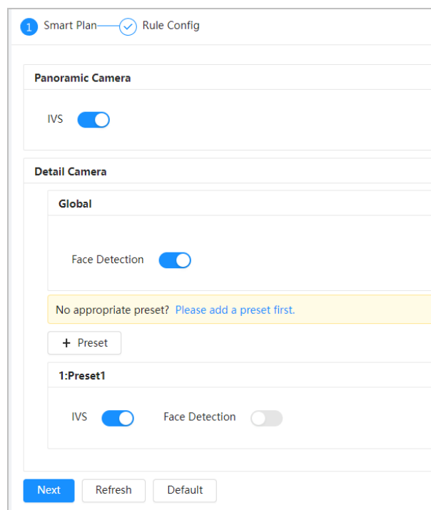
Figure 8-9 Configure smart plan (IVS)
