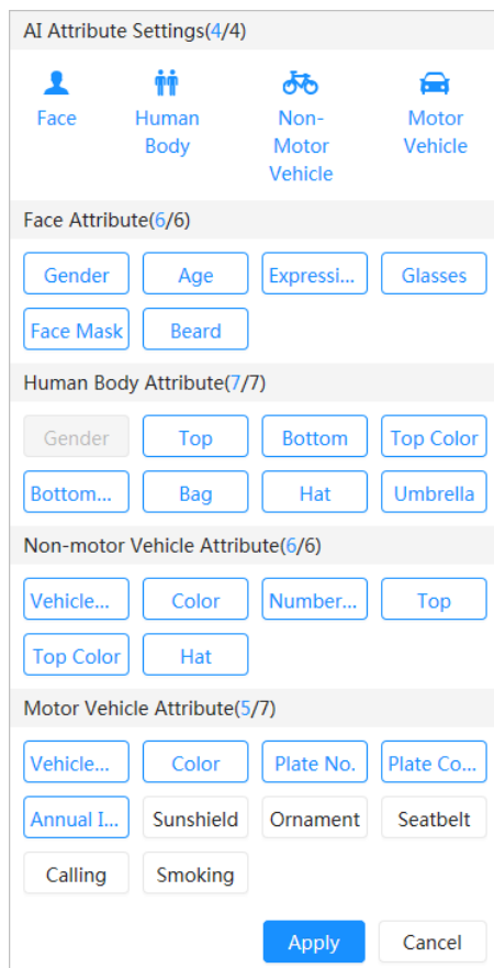
Figure 5-10 Configuring detection properties (metadata mode)
