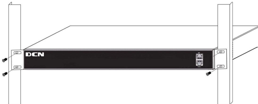
Figure 2-2 The figure of switch installing on the rack by using the front and back horn iron Caution!
